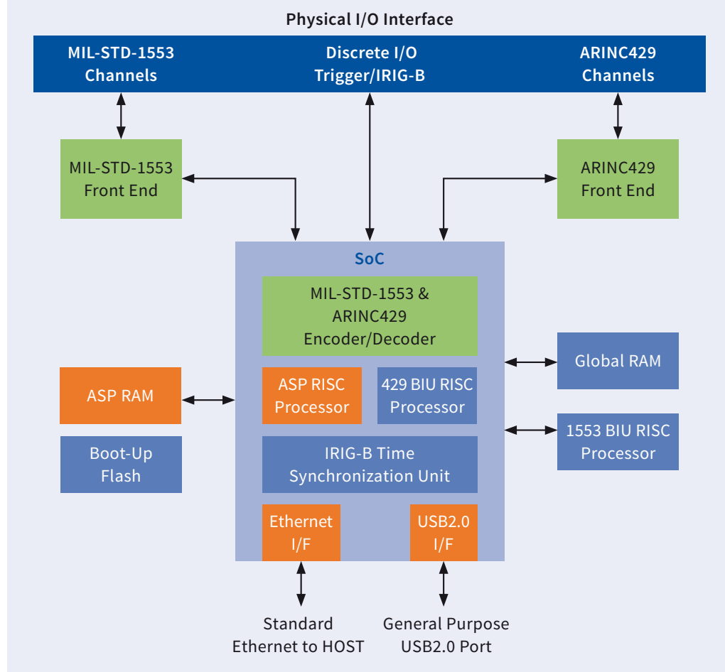
ANET-MxAy Block Diagram
