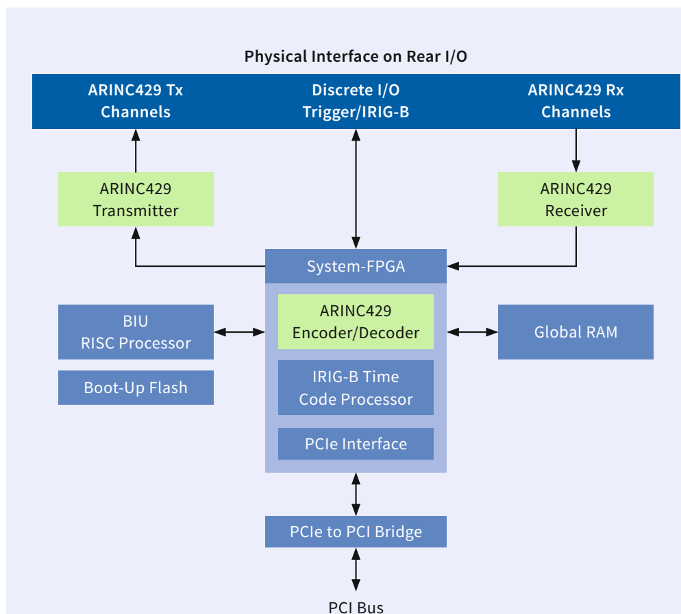
AMCE429-x Block Diagram
