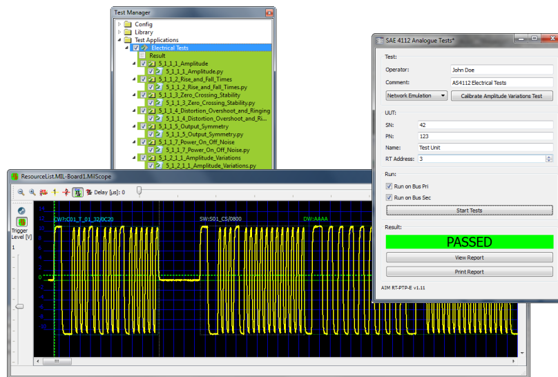
Figure 3: 1553 RT Validation Testing
