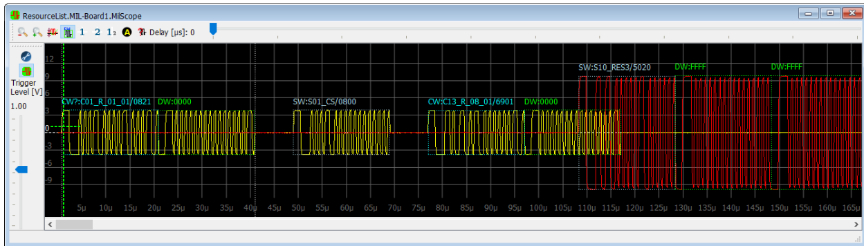
Figure 2: 1553 Message Suppression
