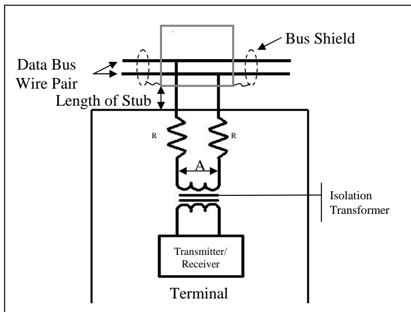
Figure 3-10 – Data Base Interface Using Direct Coupling
