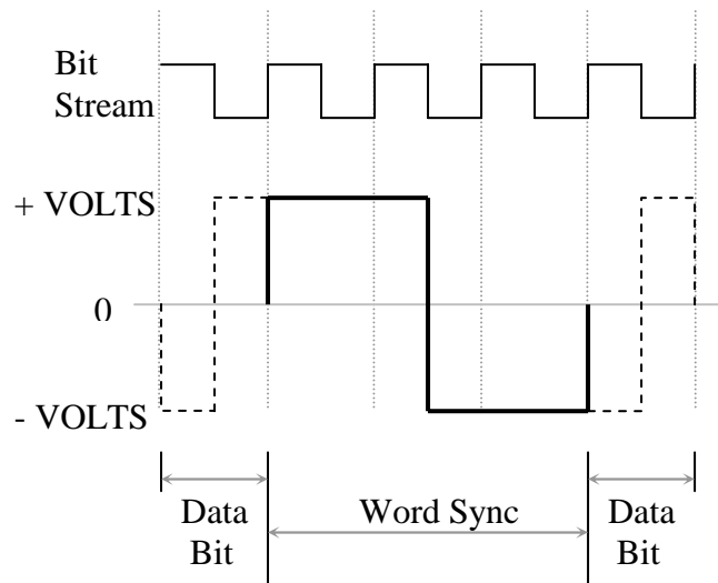
Figure 3-4 – Command and Status Sync
