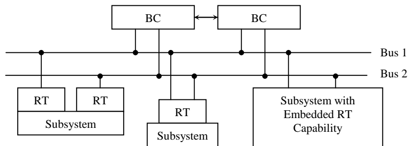
Figure 3-10.2 – Possible Redundancy
