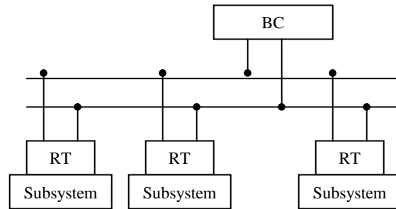
Figure 3-10.1 – Possible Redundancy
