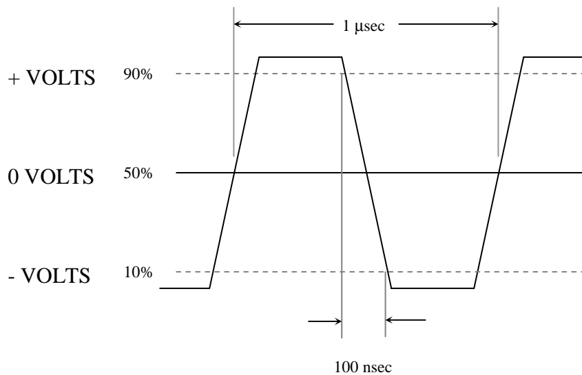
Figure 3-13 – Output Waveform
