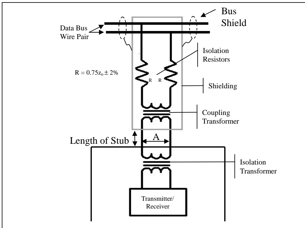
Figure 3-9 – Data Bus Interface Using Transformer Coupling
