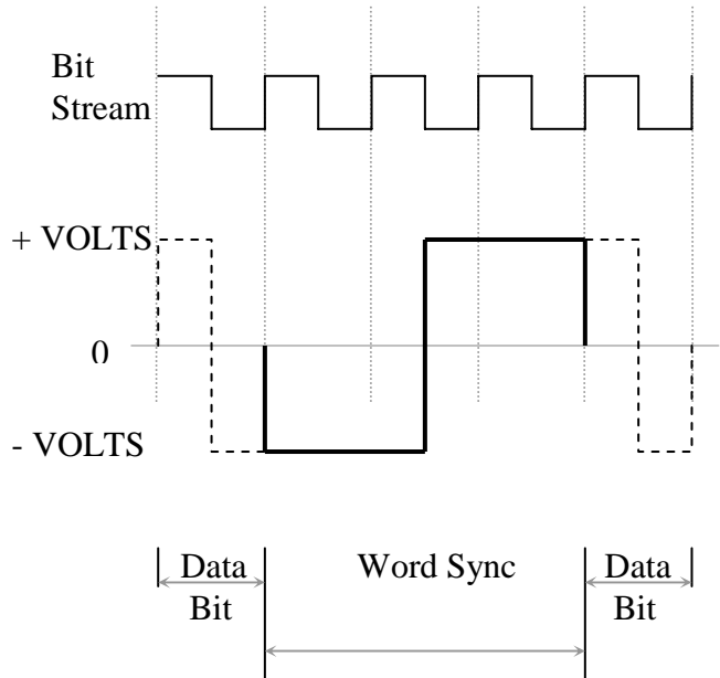
Figure 3-5 – Data Sync
