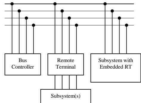
Figure 3-1 – Bus Components
