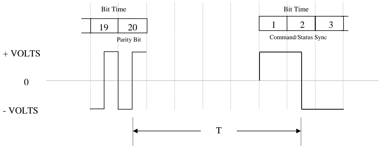
Figure 3-8 – Intermessage Gap and Response Time
