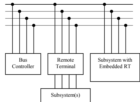
Figure 3-1 – Bus Components
